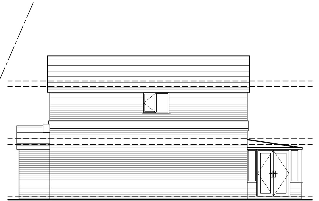
SIDE ELEVATION 1:100
