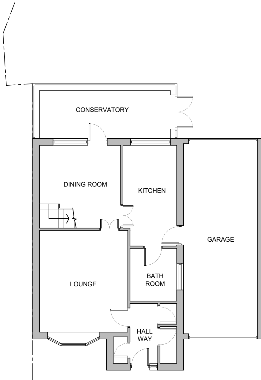
GROUND FLOOR 1:100
