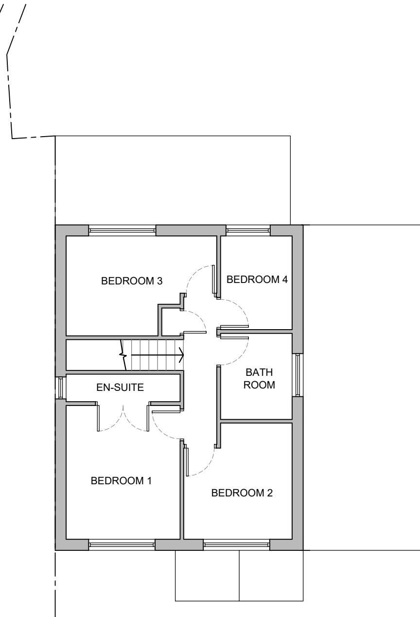
FIRST FLOOR 1:100
