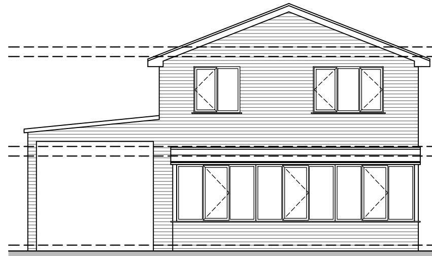
REAR ELEVATION 1:100
