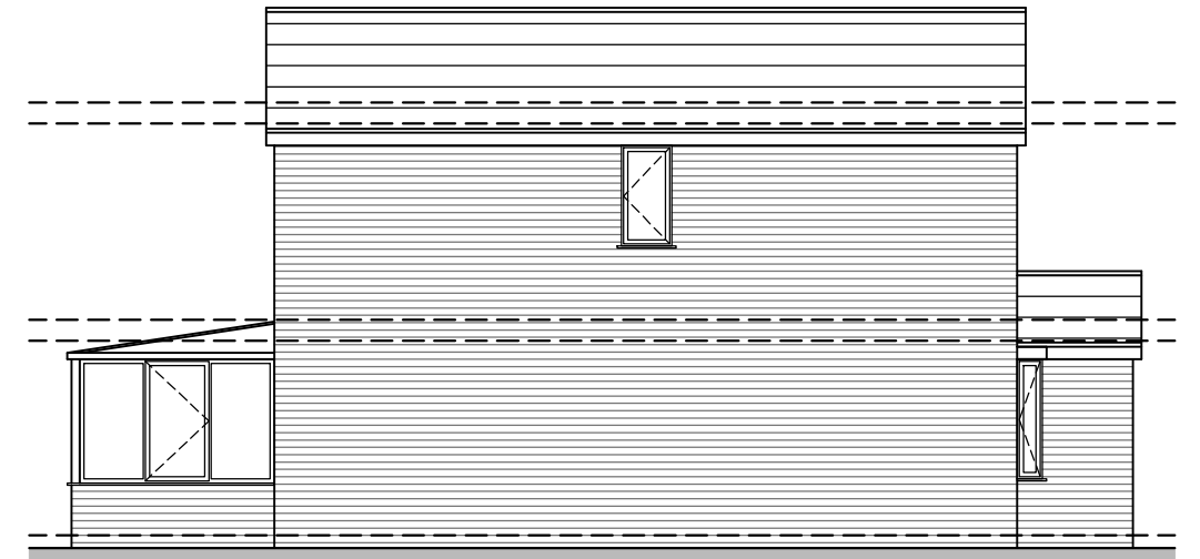
SIDE ELEVATION 1:100
